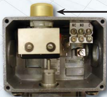
C-Series w/ Manual Reset Option (Cutaway)
