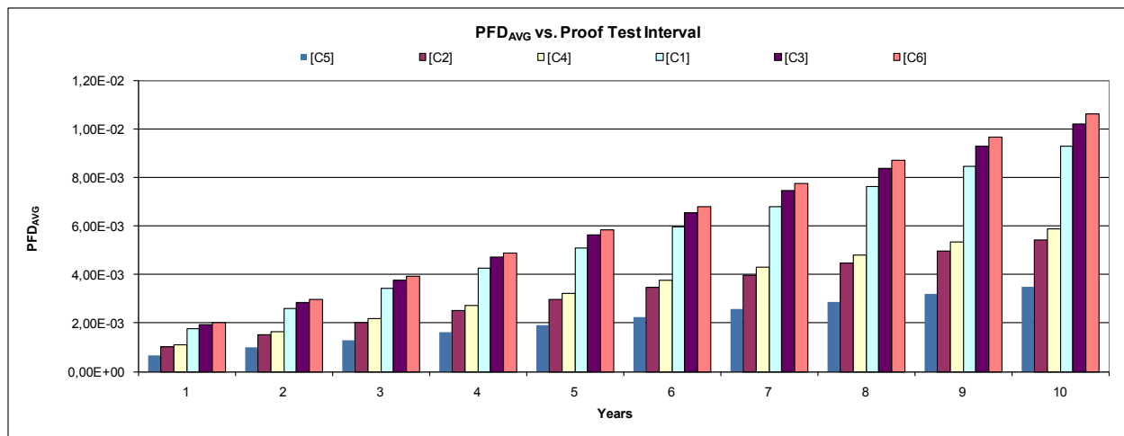
Figure 5: PFD AVG (t)
